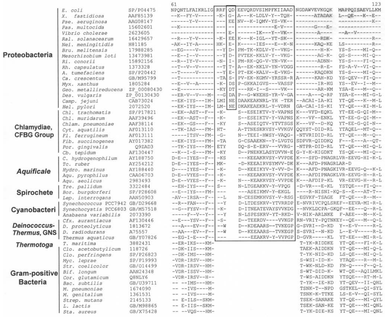
Fig. 1. Partial alignment of Hsp70 sequences showing a signature sequence consisting of an insert of 21–23-amino-acid (aa) (outer box), which is specific for diderm (characterized by the presence of an outer membrane) bacteria which comprise mainly gram-negative phyla. The smaller 2-aa insert (inner box) within the large insert is distinctive of the proteobacterial group. Dashes in the alignment indicate sequence identity with the amino acids found in Escherichia coli sequence shown on the top line. The accession numbers of various sequences are shown in the second column. Only representative sequences from different Bacteria are shown. The absence of the large insert in Aquificales species supports their placement within the diderm (gram-negative) bacteria. Abbreviations of species names are: A. , Agrobacterium ; Aqu. , Aquifex ; Bac. , Bacillus ; Bif. , Bifidobacterium ; Bor. , Borrelia ; Bru. , Brucella ; C. , Calderobacterium ; Ca. , Caulobacter ; Camp. , Campylobacter ; Cb. , Chlorobium ; Chl. , Chlamydia ; Chlam. , Chlamydomonada ; Cfx. , Chloroflexus ; Clo. , Clostridium ; Cor. , Corynebacterium ; Cyt. , Cytophaga ; D. , Deinococcus ; Des. , Desulfovibrio ; E. , Escherichia ; Fib. , Fibrobacter ; Fl. , Flavobacterium ; Geo. , Geobacter ; Hel. , Helicobacter ; Hydro. , Hydrogenothermus ; L. , Lactococcus ; Lep. , Leptospira ; M. , Mycoplasmata ; Myc. , Mycobacterium ; Myx. , Myxococcus ; Nei. , Neisseria ; Pas. , Pasteurella ; Por. , Porphyromonas ; Pse. , Pseudomonas ; Ral. , Ralstonia ; Ri. , Rickettsia ; Rh. , Rhodobacter ; Sta. , Staphylococcus ; Str. , Streptomyces ; Strep. , Streptococcus ; T. , Thermotoga ; Tc. , Thermocrinis ; Tre. , Treponema ; X. , Xyella . GNS in bacterial groups name refers to green nonsulfur bacteria ( Cfx. aurantiacus ).
