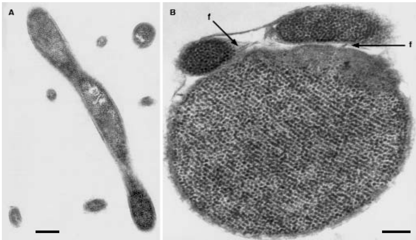
Fig. 2 Spirosymplokos deltaeiberi from Spain, electron micrographs. (A) Single (noncomposite) Ebro delta spirochete with 5-10-5 (or 6-12-6) flagella insertions in longitudinal and (upper right) tranverse section. Both continuity of flagella with cytoplasmic granules and density of the array of granules are clearly seen; bar = 5 \mu\text{m} . (B) Composite Ebro delta spirochete in membrane-bounded round body that shows typical low number of periplasmic flagella (f), packed arrays of protoplasmic-cylinder granules and variable diameter; bar = 1 \mu\text{m}
