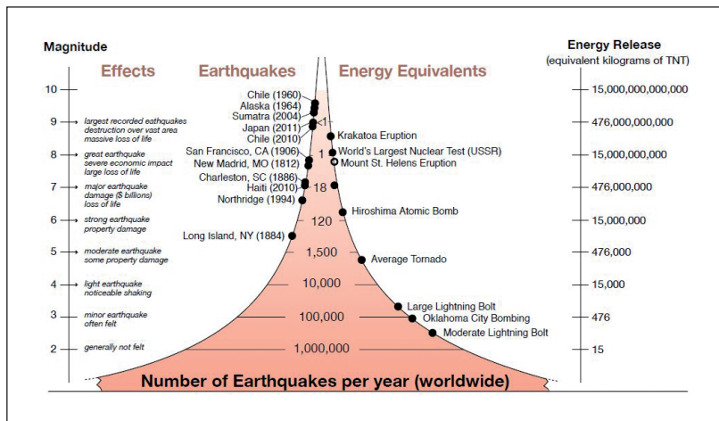
Fig. 4. Worldwide number of earthquakes per year, and energy equivalences. © The Iris Consortium. Education and outreach series, n°. 3.
