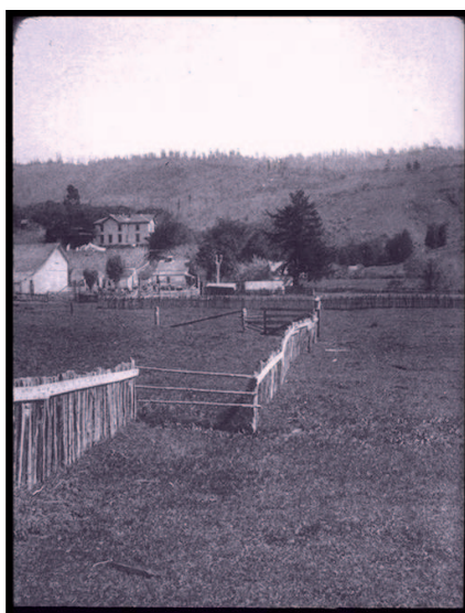
Fig. 2. A 2.5-m displacement of a fence, near Point Reyes, California, produced along the fault during the 1906 San Francisco earthquake. Photo: by G.K. Gilbert.
