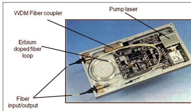
Fig. 7. Erbium-doped fiber amplifier (EDFA).
