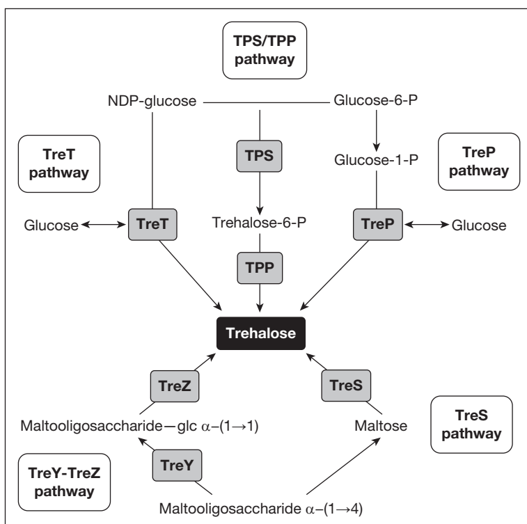
Fig. 2. Pathways for the synthesis of trehalose. TPS, trehalose-6-phosphate synthase; TPP, trehalose-6-phosphate phosphatase; TreS, trehalose synthase; TreY, maltoligosyl-trehalose synthase; TreZ, maltoligosyl-trehalose trehalohydrolyase; TreP, trehalose phosphorylase; TreT, trehaloseglycosyl-transferring synthase.
