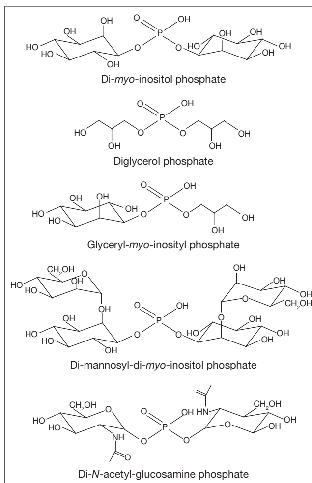
Fig. 3. Structure of known phosphodiester compatible solutes, primarily found in hyperthermophilic organisms.
