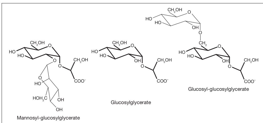
Fig. 4. Structure of glucosylglycerate and of the naturally occurring derivatives glucosyl-glycosylglycerate and mannosyl-glycosylglycerate.
