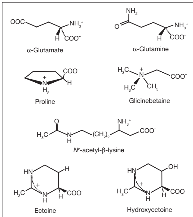
Fig. 1. Structure of some naturally occurring amino acid compatible solutes and amino acid derivatives.
