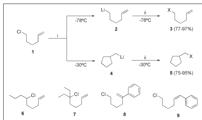
Fig. 1. Reagents: (i) Li, DTBB (5%), THF; (ii) electrophile = Bu t CHO, PhCHO, Et 2 CO, (CH 2 ) 5 CO, PhCOMe, then HCl-H 2 O.
