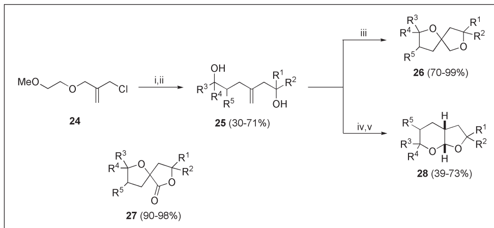
Fig. 4. Reagents: (i) Li, C_{10}H_8 (2.5%), R^1R^2CO = Et_2CO, (CH_2)_4CO, (CH_2)_5CO, O(CH_2CH_2)_2CO , adamantan-2-one, THF, -78 to 0^\circ C ; (ii) R^3R^4C(O)CHP^5 = MeCH(O)CH_2, PhCH(O)CH_2, n-C_6H_{13}CH(O)CH_2, Et_2C(O)CH_2, PhMeC(O)CH_2, (n-C_5H_{11})_2C(O)CH_2 , cyclopentene oxide, cyclohexene oxide, methylenecyclohexane oxide, methyleneadamantane oxide, 0^\circ C , then H_2O ; (iii) I_2, Ag_2O , THF; (iv) BH_3 \cdot THF , then H_2O_2 \cdot NaOH ; (v) PCC or Ru(PPh_3)_3Cl_2, CH_2Cl_2 .
