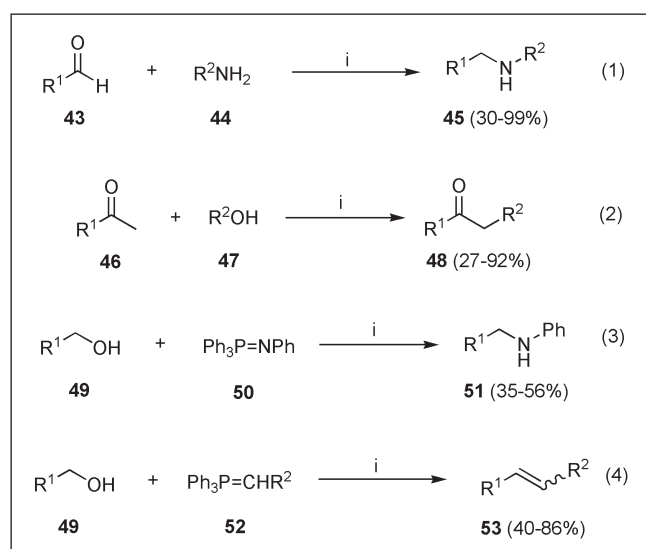
Fig. 7. Reagents: (i) NiCl 2 , 2Li, DTBB (5%), solvent [PrOH reflux (1) or THF at room temperature (2) or at reflux (3), (4)].
