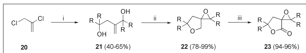
Fig. 4. Reagents: (i) Li, C_{10}H_8 (2.5%), R^1R^2CO = Et_2CO, (CH_2)_4CO, (CH_2)_5CO, O(CH_2CH_2)_2CO , adamantan-2-one, THF, -78 to 0^\circ C ; (ii) R^3R^4C(O)CHP^5 = MeCH(O)CH_2, PhCH(O)CH_2, n-C_6H_{13}CH(O)CH_2, Et_2C(O)CH_2, PhMeC(O)CH_2, (n-C_5H_{11})_2C(O)CH_2 , cyclopentene oxide, cyclohexene oxide, methylenecyclohexane oxide, methyleneadamantane oxide, 0^\circ C , then H_2O ; (iii) I_2, Ag_2O , THF; (iv) BH_3 \cdot THF , then H_2O_2 \cdot NaOH ; (v) PCC or Ru(PPh_3)_3Cl_2, CH_2Cl_2 .
