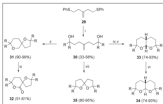
Fig. 5. Reagents: (i) Li, DTBB (2.5%), R_2CO = Et_2CO, Pr^i_2CO, Bu^t_2CO, (n-C_5H_{11})_2CO, (c-C_3H_5)_2CO, (CH_2)_4CO, (CH_2)_5CO, Y(CH_2CH_2)_2CO [ Y = O, S, Pr^iN ], adamantan-2-one, THF, 0^\circ C , then H_2O ; (ii) I_2, AgOTf , THF; (iii) NaIO_4, RuO_2 (cat.), CCl_4 ; (iv) BH_3 \cdot THF , then H_2O_2 \cdot NaOH ; (v) PCC, CH_2Cl_2 ; (vi) p -TSA, CHCl_3 ; (vii) O_3, CH_2Cl_2, -78^\circ C .
