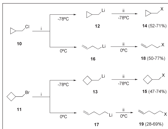
Fig. 2. Reagents: (i) Li, DTBB (for 10 ) or C 10 H 8 (for 11 ) (5%), THF; (ii) electrophile = Pr i CHO, Bu t CHO, PhCHO, Et 2 CO, Pr n 2 CO, ( c -C 3 H 5 ) 2 CO, (CH 2 ) 5 CO, PhCOMe, then H 2 O.
