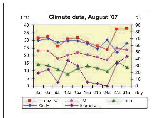
Fig. 4. Temperatures (maximum, minimum, average) and relative humidity of August 2007. Increased T calculated as percentage of the increment considering the lowest temperature average ( 16.8^{\circ}\text{C} ).
