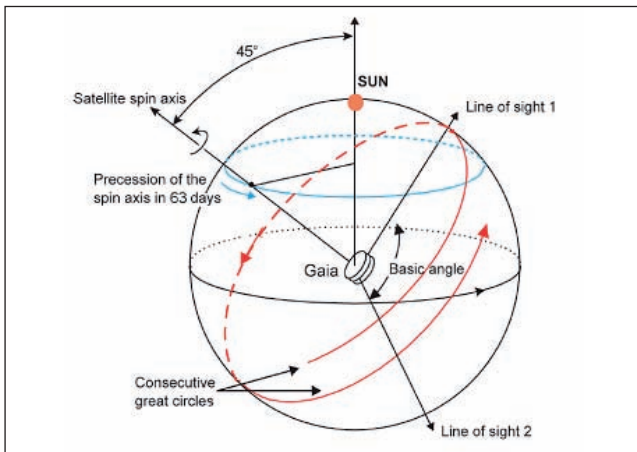
Fig. 3. Gaia's two astrometric fields of view scan the sky according to a carefully prescribed revolving scanning law. The constant spin rate of 60 arcsec/s corresponds to 6-hour great-circle scans. The angle between the slowly precessing spin axis and the sun is maintained at 45°. The basic angle between the two lines of sight is 106.5°. (Courtesy of Karen O'Flaherty).
