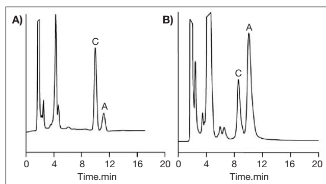
Fig. 6. Chromatograms of ( A ) a minced beef sample diluted 1:10 and ( B ) a chicken and turkey hamburger sample diluted 1:1 . A, Anserine, C carnosine. (Reproduced with the permission of Elsevier [14]).
