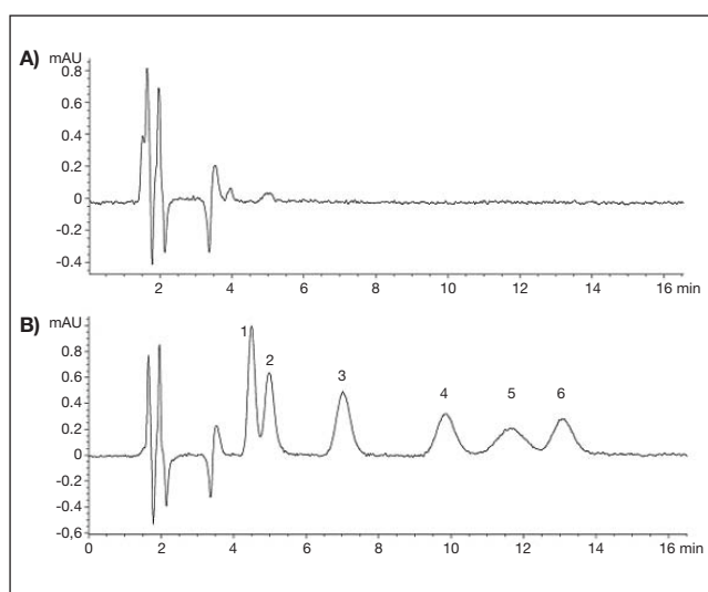
Fig. 8. Chromatograms obtained from milk samples: (A) blank milk treated with the diazotization-coupling reagents, with the azo-dye visualized at 490 nm; (B) milk spiked with 25 ng/ml of each sulfonamide. Sulfonamides and retention times (min) were: (1) sodium sulfacetamide, 4.5, (2) sulfamethizole, 5.0, (3) sulfaguandinine, 7.0, (4) sulfamerazine, 9.9, (5) sulfathiazole, 11.6, and (6) sulfamethoxazole, 13.2. (Reproduced with the permission of Elsevier [21].)
