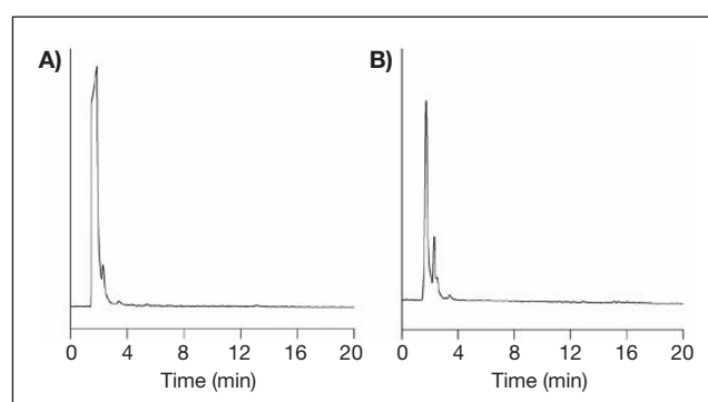
Fig. 3. Micellar liquid chromatograms in which the serum (A) and urine (B) blanks have been directly injected into the chromatograph.
