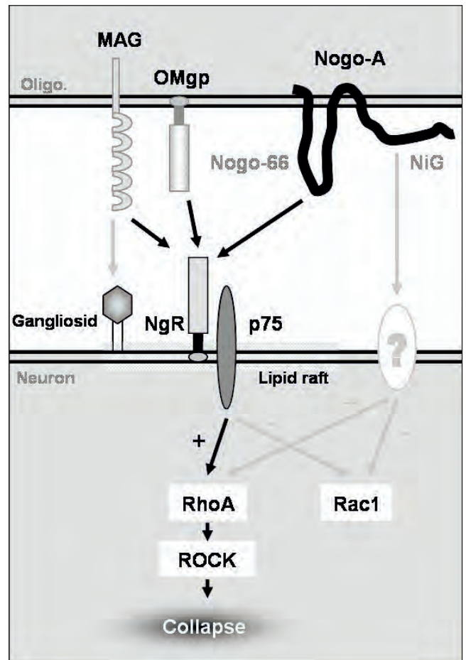
Figure 3. Schematic representation of the proposed interactions between NgR and its ligands. Black arrows symbolize well established interactions; grey arrows correspond to supposed interactions. Nogo-66, MAG and OMgp bind to NgR, and its association with p75 activates Rho and ROCK, leading to the growth cone collapse. In addition, interaction of MAG with gangliosids may facilitate NgR-p75 binding. The putative neuronal NiG receptor and the subsequent activation of Rho and inhibition of Rac by NiG binding are also represented in this figure. Although the complete receptor complex is formed by NgR, p75 or Troy and Lingo-1, only p75 has been represented. Abbreviations: MAG, myelin-associated glycoprotein; NgR, Nogo receptor; Oligo., oligodendrocyte; OMgp, oligodendrocyte myelin glycoprotein; ROCK, Rho-kinase.
